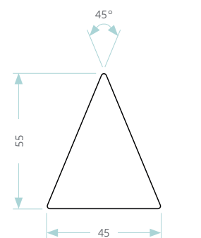
Triangle Batten for 135° Bay
