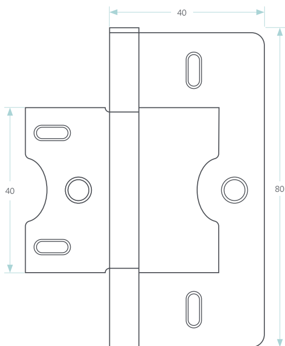
SELF MORTICE HINGE
